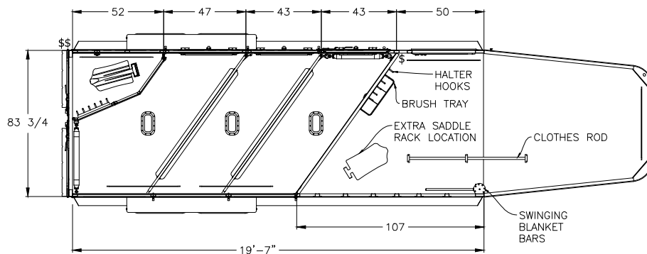
Floorplan shown: 3H with 50" dressing room.
