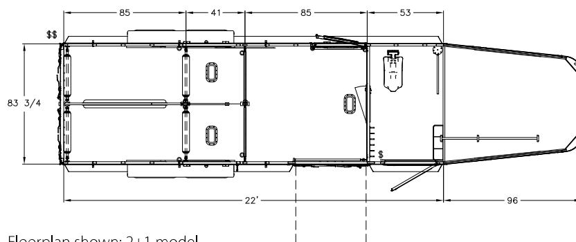
Floorplan shown: 2+1 model.
