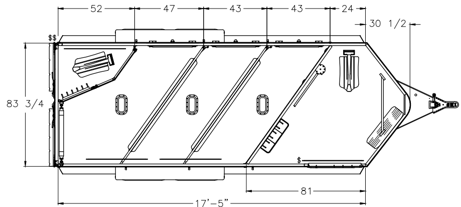
Floorplan shown: 3H with 24" dressing room.
