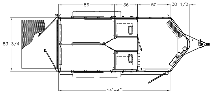
Floorplan shown: 50" with walk thru door.
